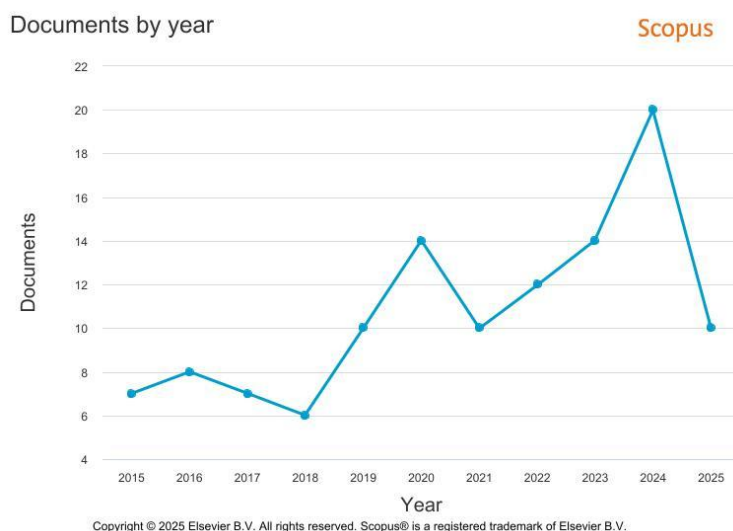
Gambar 1. Analisis Bibliometrik Documents by Year
