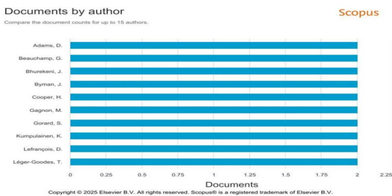
Gambar 4. Analisis Bibliometrik Documents By Author
