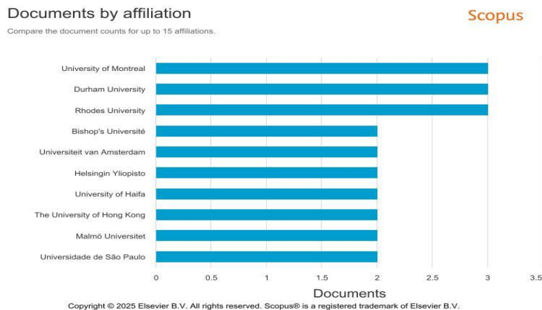
Gambar 3. Analisis Bibliometrik Documents By Affiliation
