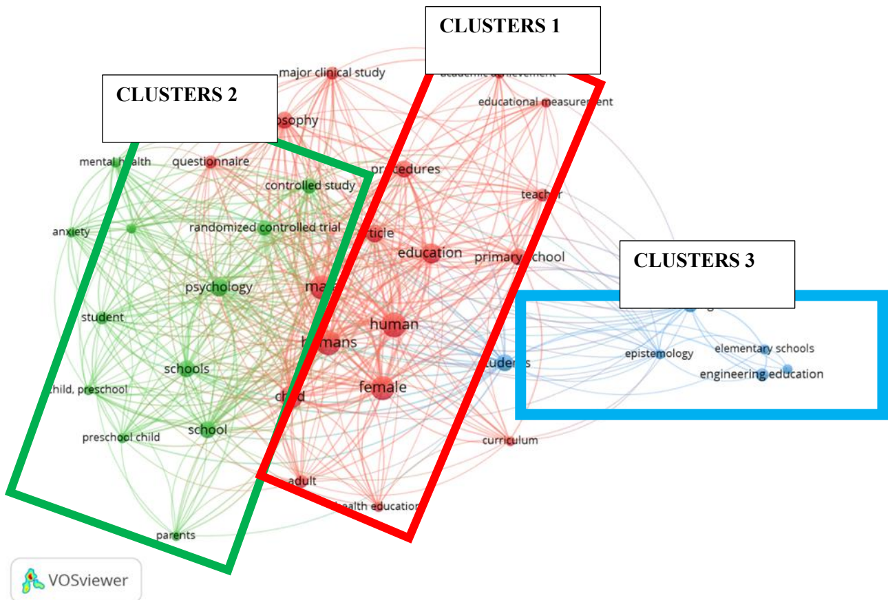
Gambar 2. Analisis Bibliometrik Co-Occurance Network Visualization
