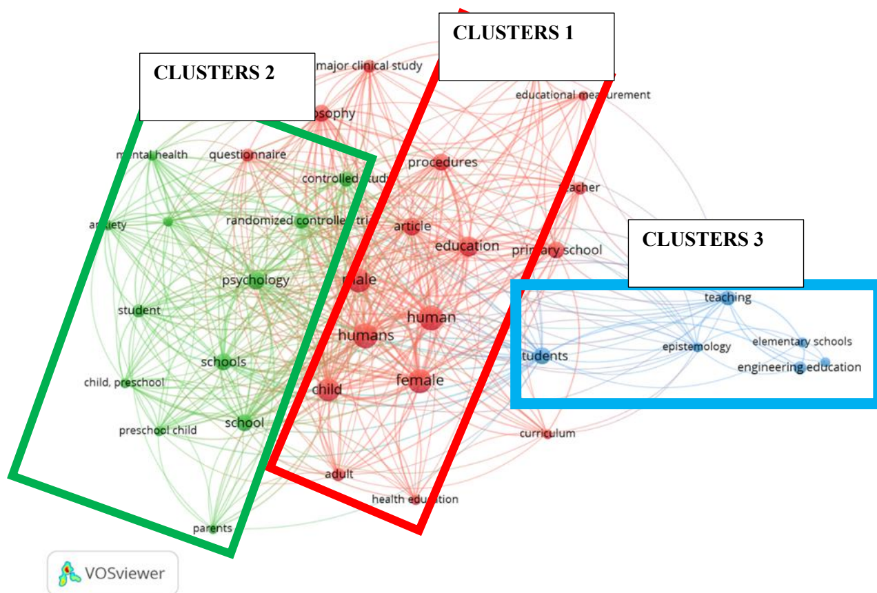
Gambar 6. Analisis Bibliometrik Co-Occurance Network Visualization
